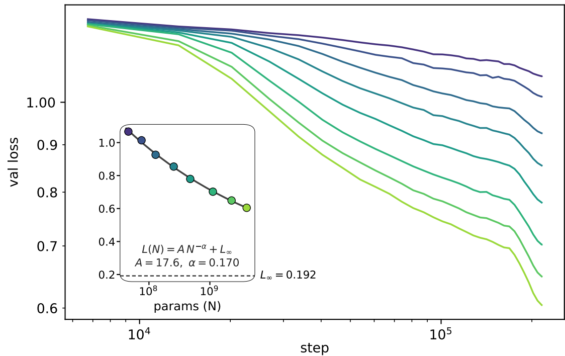
Parameter scaling — loss curves & scaling law N = 46\text{M} - 4\text{B} , D = 84\text{B} , C = 2.5 \times 10^{19} - 2.1 \times 10^{21}
