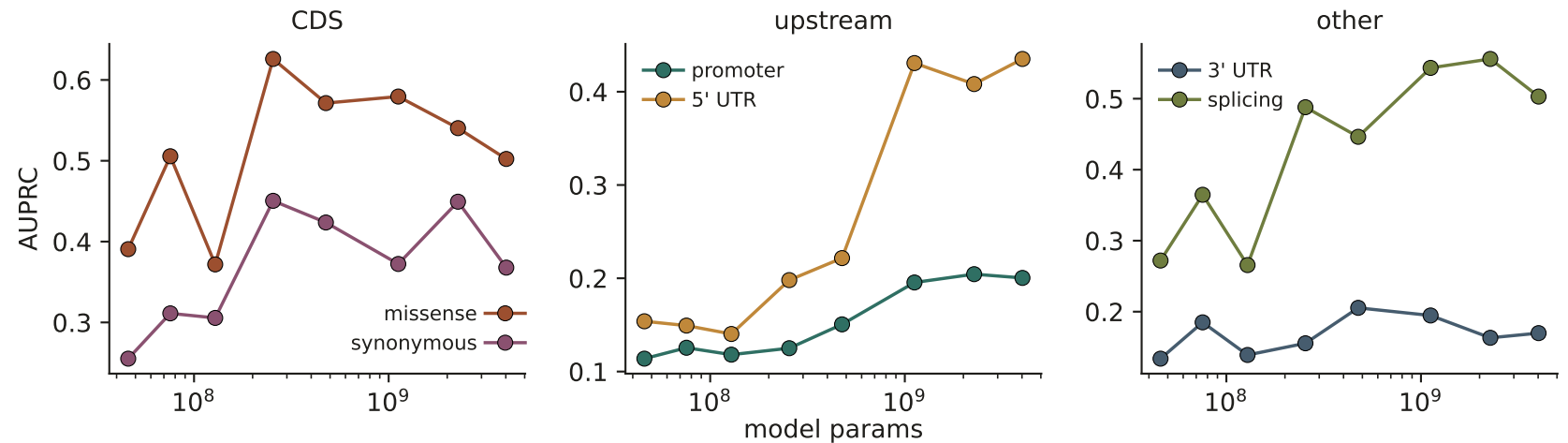
Parameter scaling — params vs VEP AUPRC by variant type
