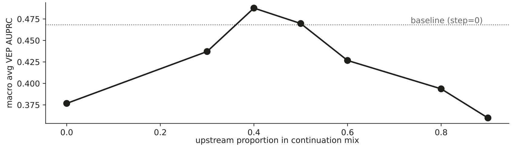
Continued pretraining from uniform mixture
