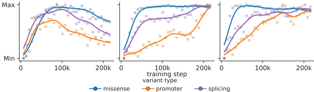
Parameter scaling — VEP AUPRC across training steps
