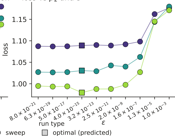
Transfer validation — loss vs \beta_2 and \varepsilon
