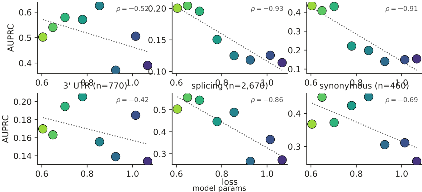
Parameter scaling — loss vs VEP AUPRC by variant type
