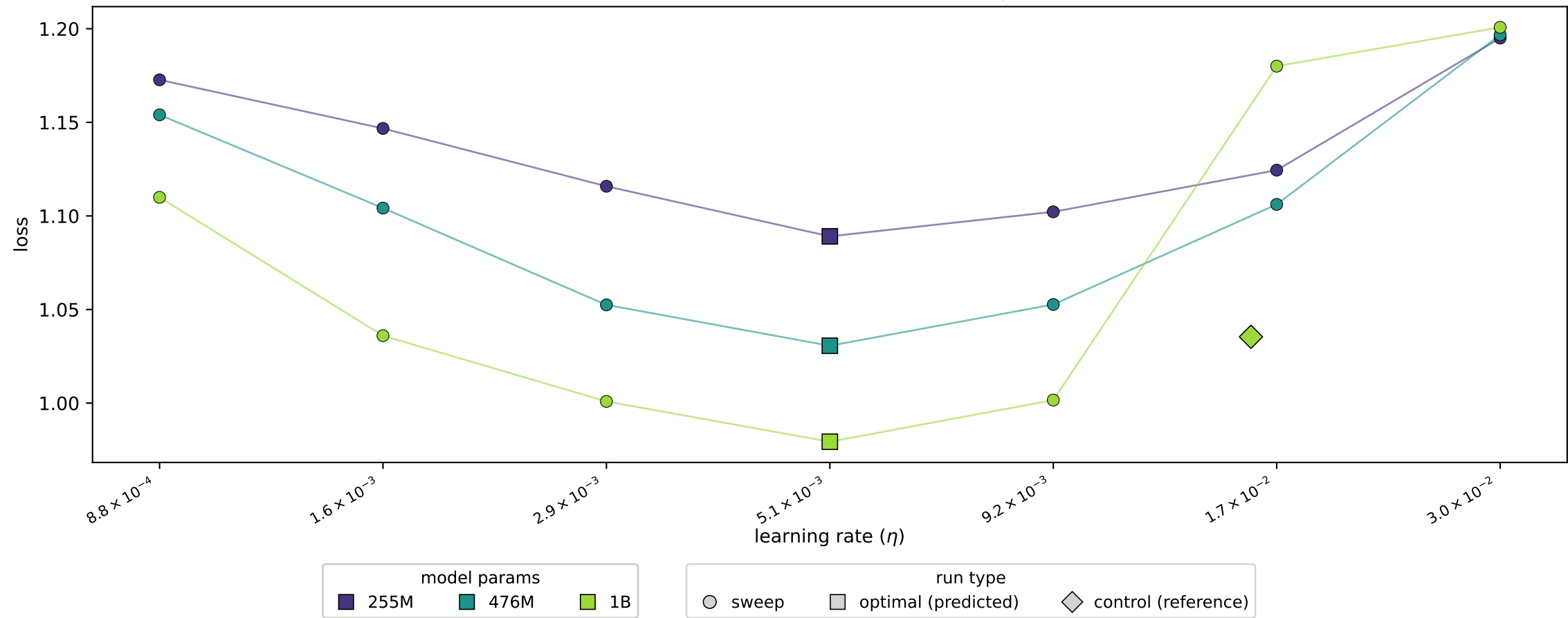
Transfer validation — loss vs learning rate
