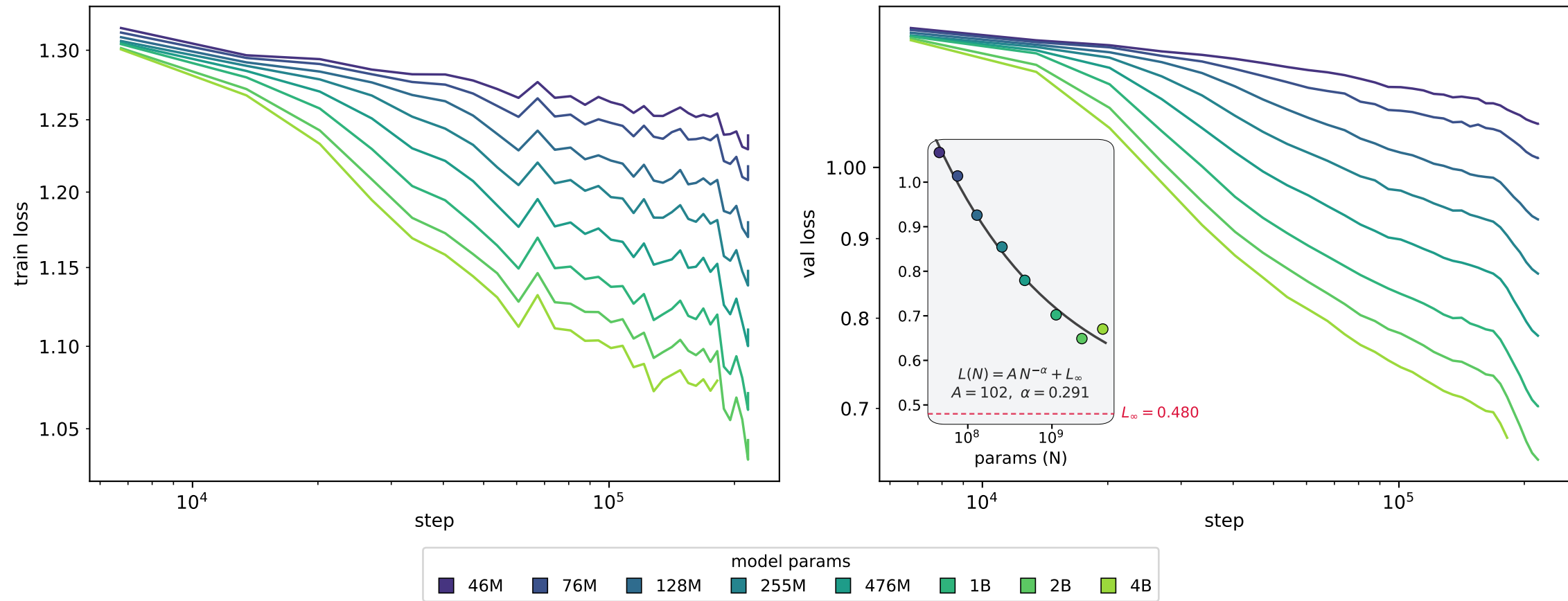
Parameter scaling — loss curves &amp; scaling law
