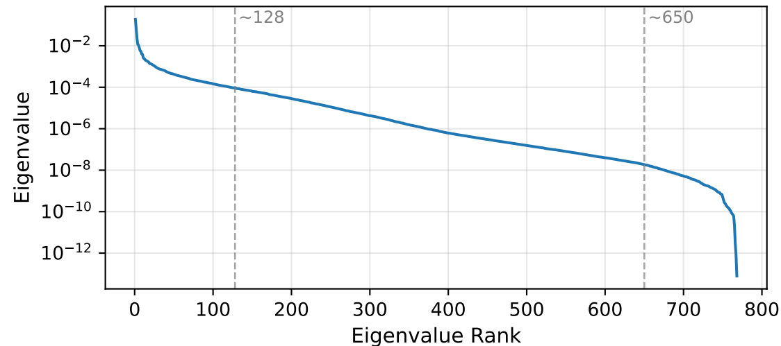
v13: PlantCAD2-S-88M 8192bp Angiosperm 2.6M 65sp (n=65,536)
