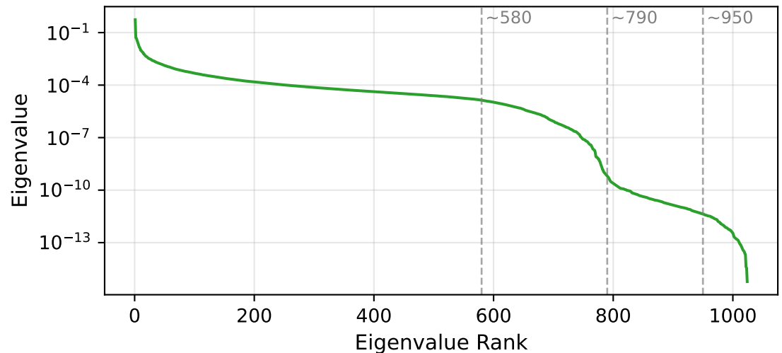
v40: GLM-Experiments-299M 512bp GPN animal promoter 417sp (n=262,144)
