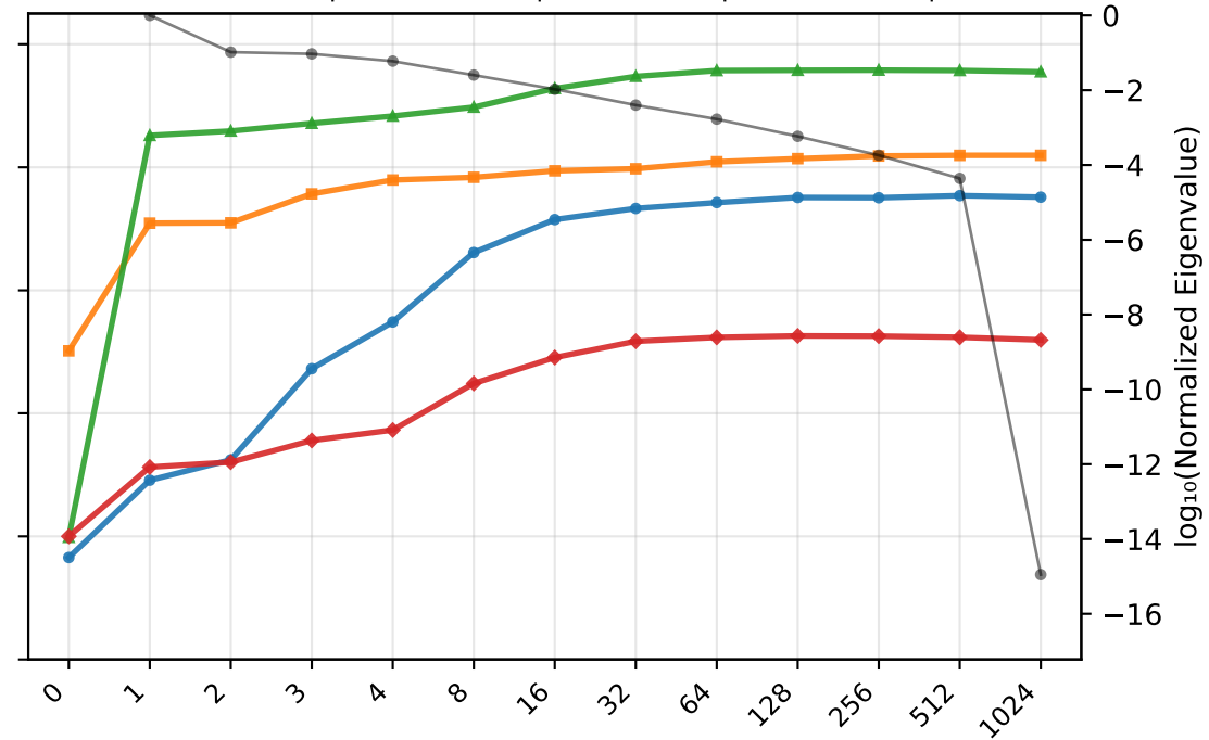
v41: GLM-Experiments 512bp GPN animal promoter 9M 6sp
