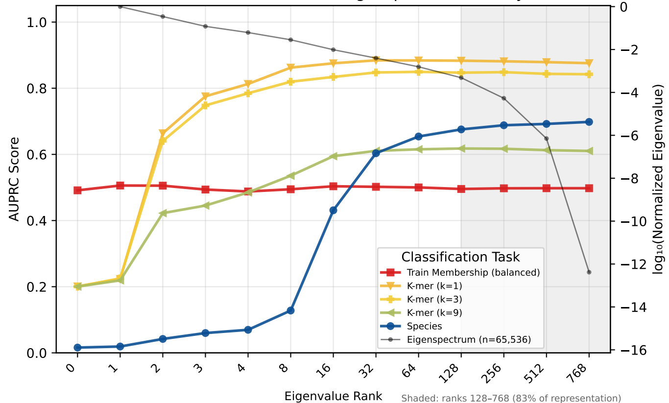
AUPRC Performance with Eigenspectrum Overlay
