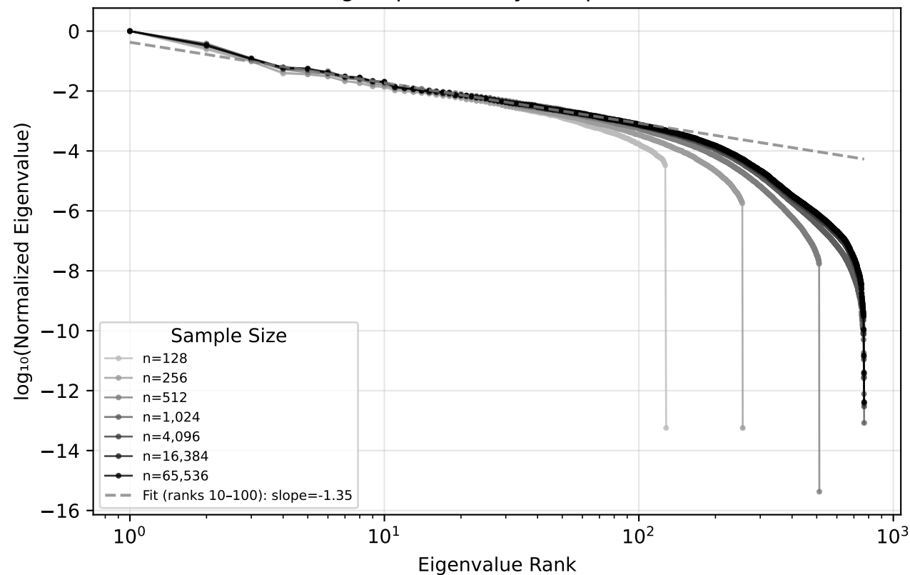
Eigenspectrum by Sample Size
