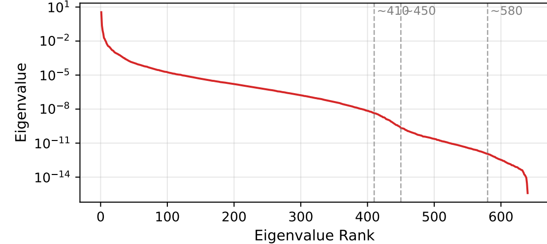
v46: Marin IsoFLOP-45M 4096bp Metagenomes (n=65,536)
