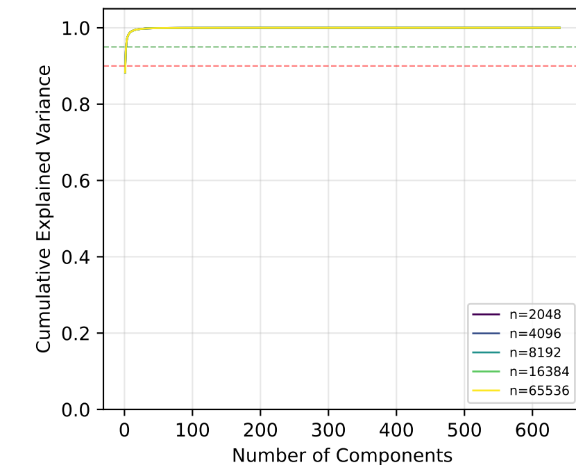
Cumulative Variance
