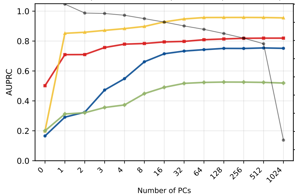
v41: GLM-Experiments-299M 512bp GPN animal promoter 9M 6sp
