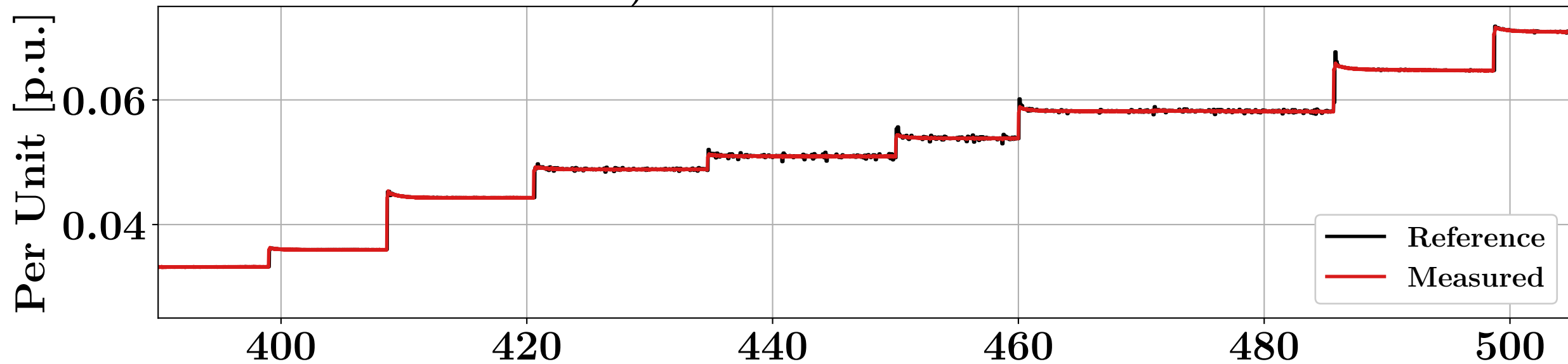
a) Active Power dVOC 1
