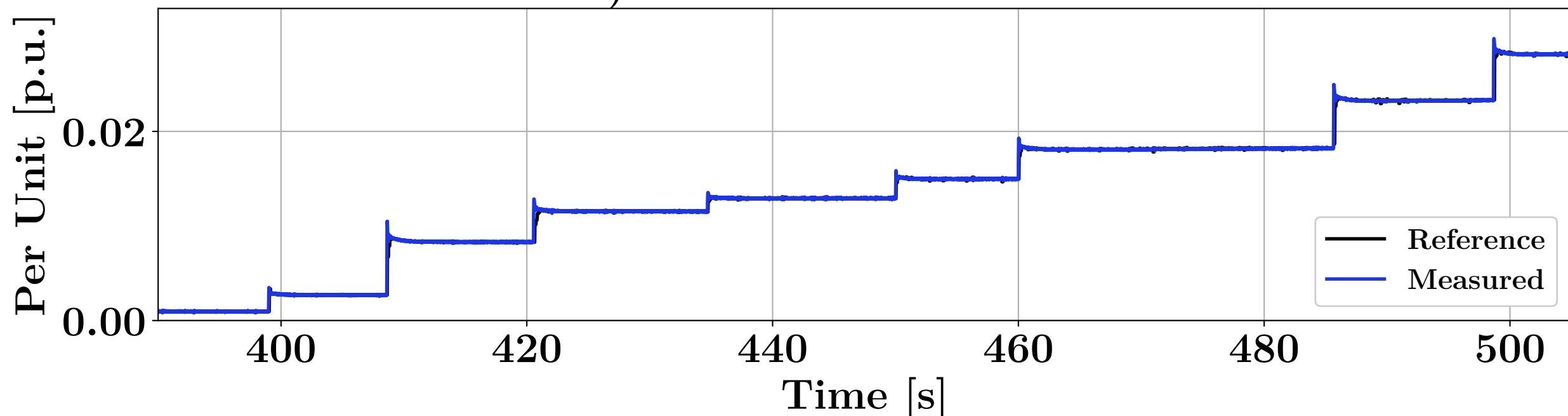
b) Reactive Power dVOC 1
