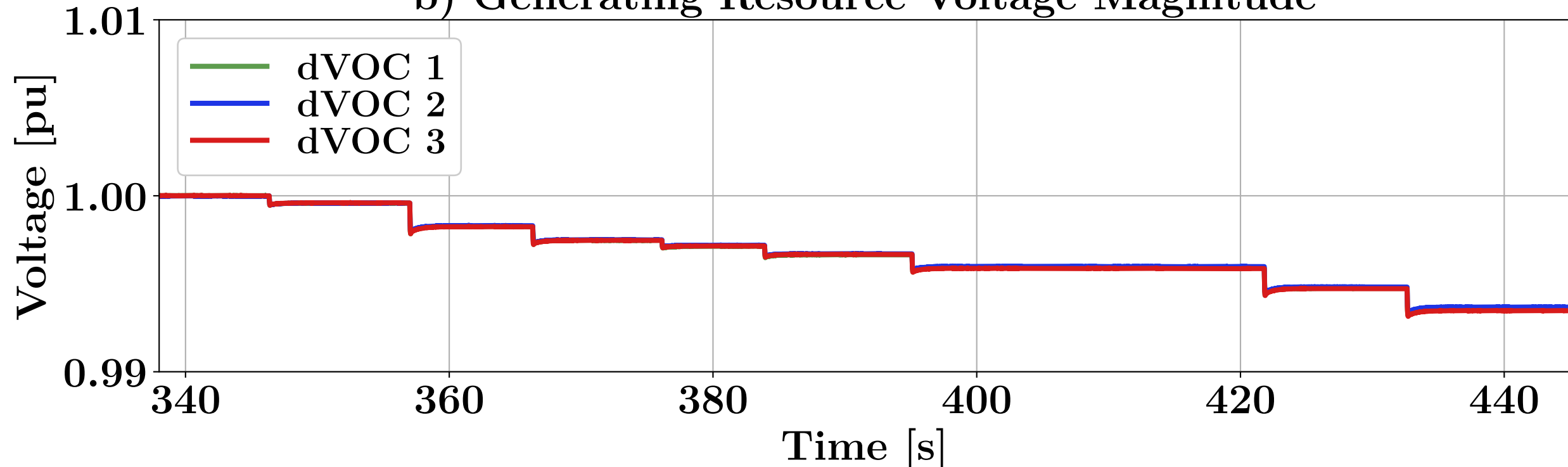
b) Generating Resource Voltage Magnitude
