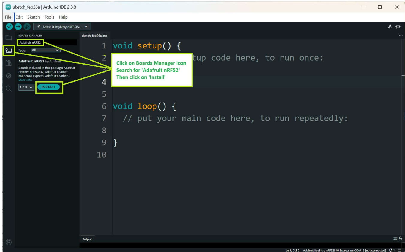
Figure 3 – Open the Arduino IDE Boards Manager & Install Adafruit nRF52
