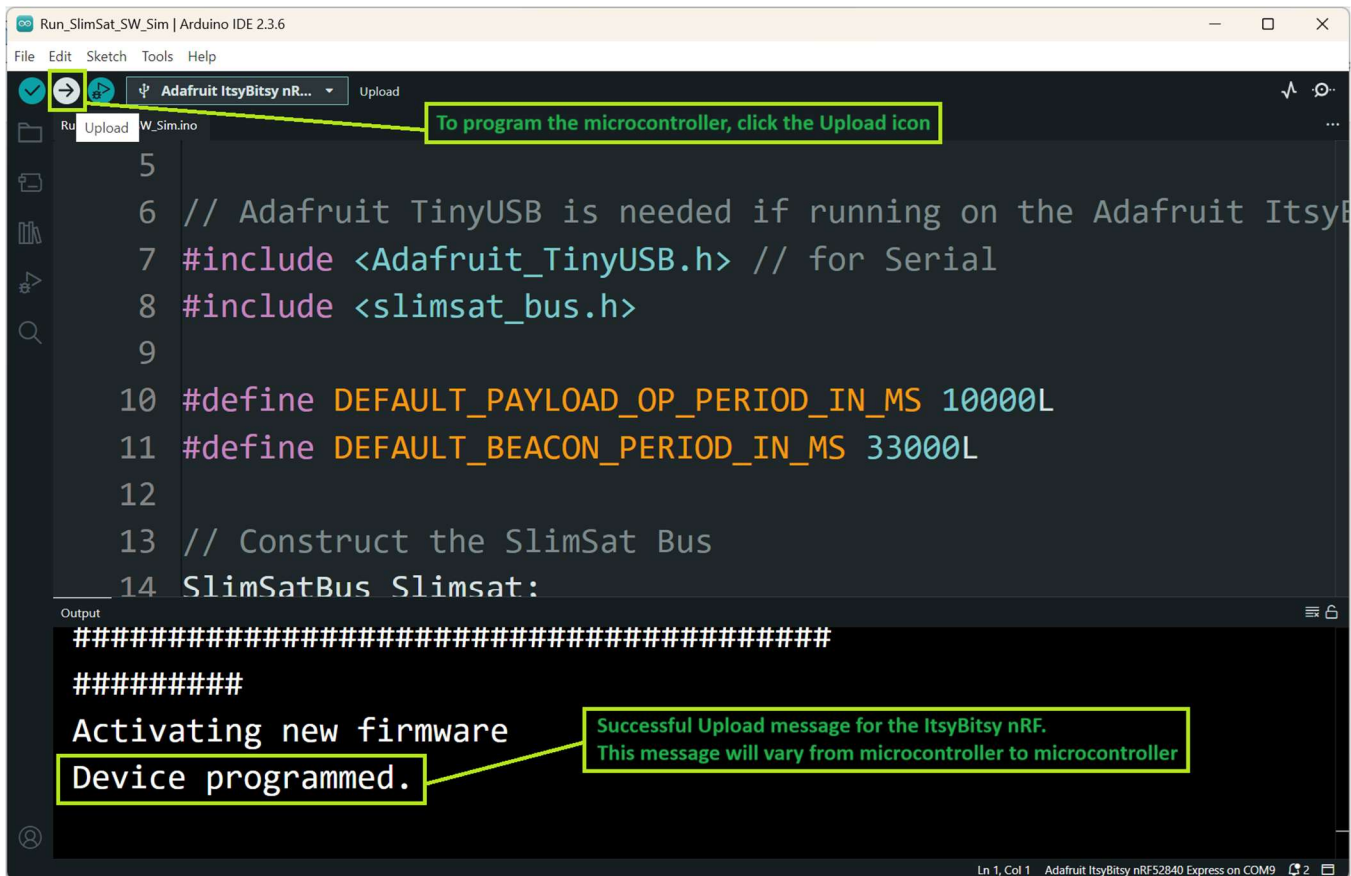
Figure 17 – Successful Upload of the Run SlimSat SW Sim Example
