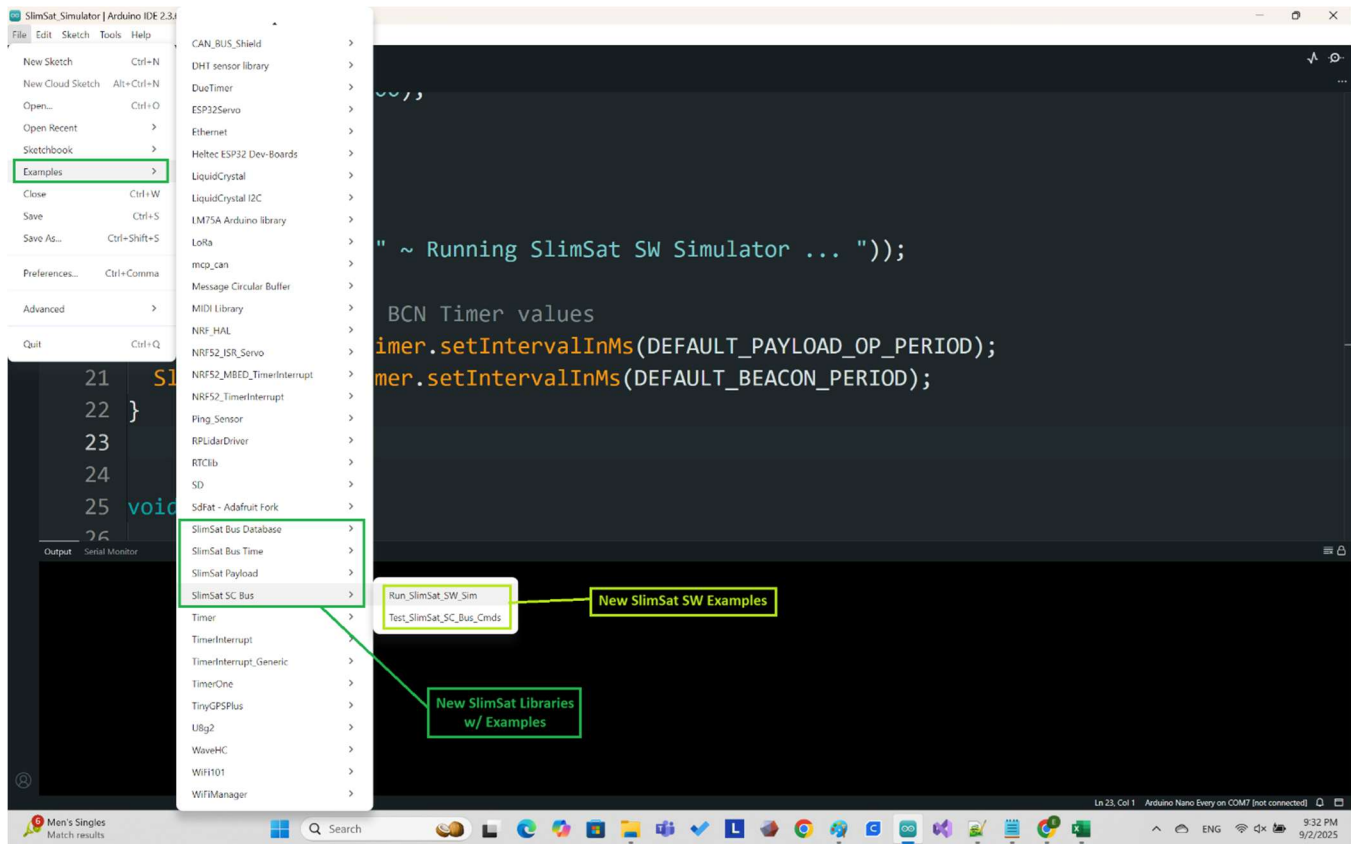
Figure 14 – In Arduino IDE, Click File -> Examples, & Navigate to Run SlimSat SW Sim Example
