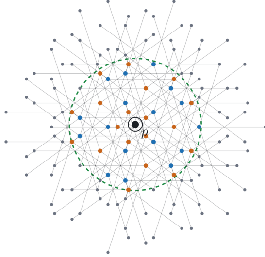
Figure 5. The point's-eye view of the orbit of a point p at r = 2 (143 positions). Each position is a pair of disk centres 2v - 1 (blue) and 2(v + \bar{m}) - 1 (orange) joined by a segment; grey centres lie outside the window (dashed circle of radius r about p ) and cannot be turned about.
