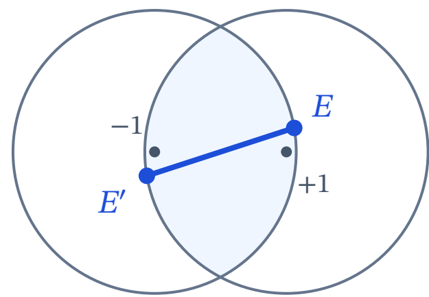
The chord E'E in the lens at r = r_c(5)
