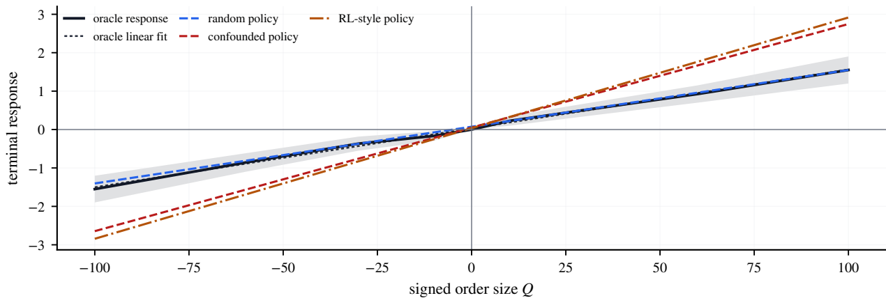
A. Price-impact response curves
