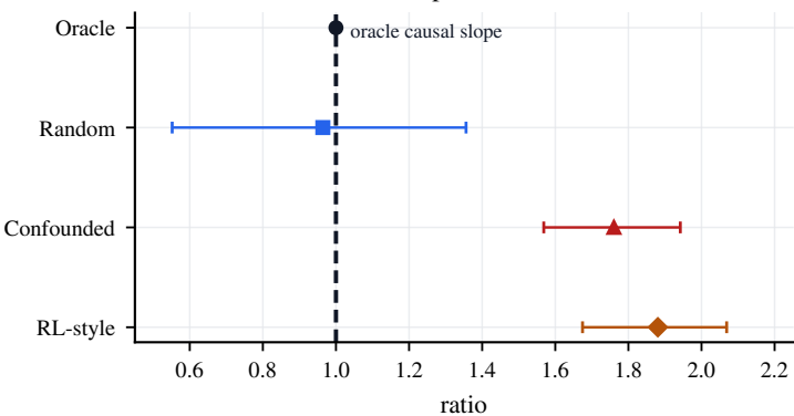
B. Slope vs oracle
