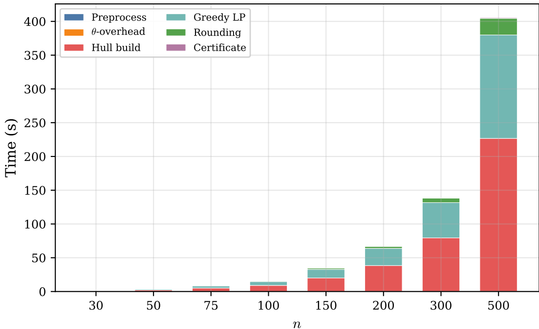
Runtime breakdown ( m = 50 )
