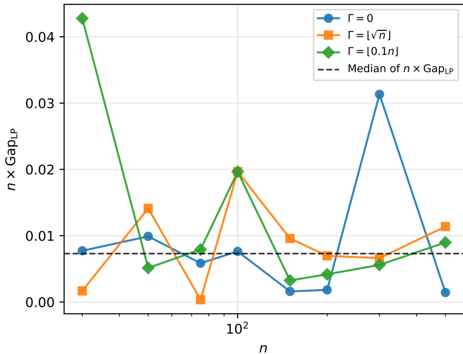
Scaled relative gap vs n
