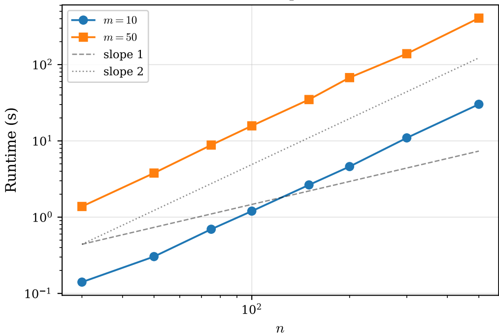
Runtime vs. prefix size
