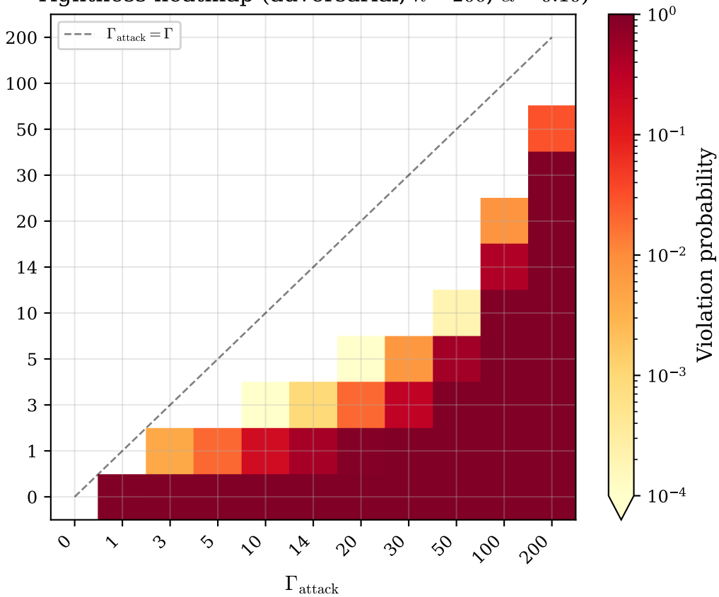
Tightness heatmap (adversarial, n = 200 , \alpha = 0.10 )
