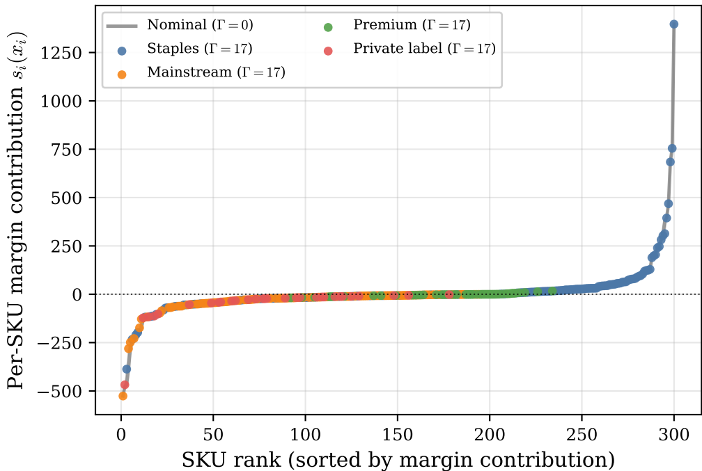
Margin distribution: nominal vs. robust
