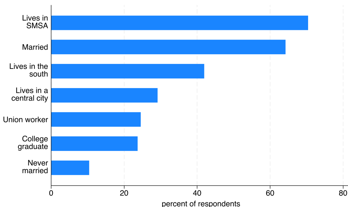
Figure 9.2: Seven indicator variables from nlswh88 as ranked percentages, drawn by one statplot call with percent sort descending wrap(12) . Metro residence leads at 70% and never-married closes at 10%; every bar label is a curated variable label, wrapped rather than abbreviated. Built by ch09_graphs.do .
