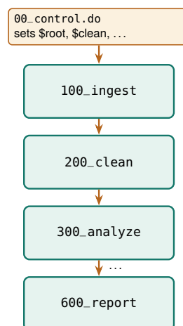
Figure 2.4: The numbered pipeline. The control file sets the paths, then sources each stage in order. Numbering by hundreds leaves room to insert a 150_ step later without renaming everything.
