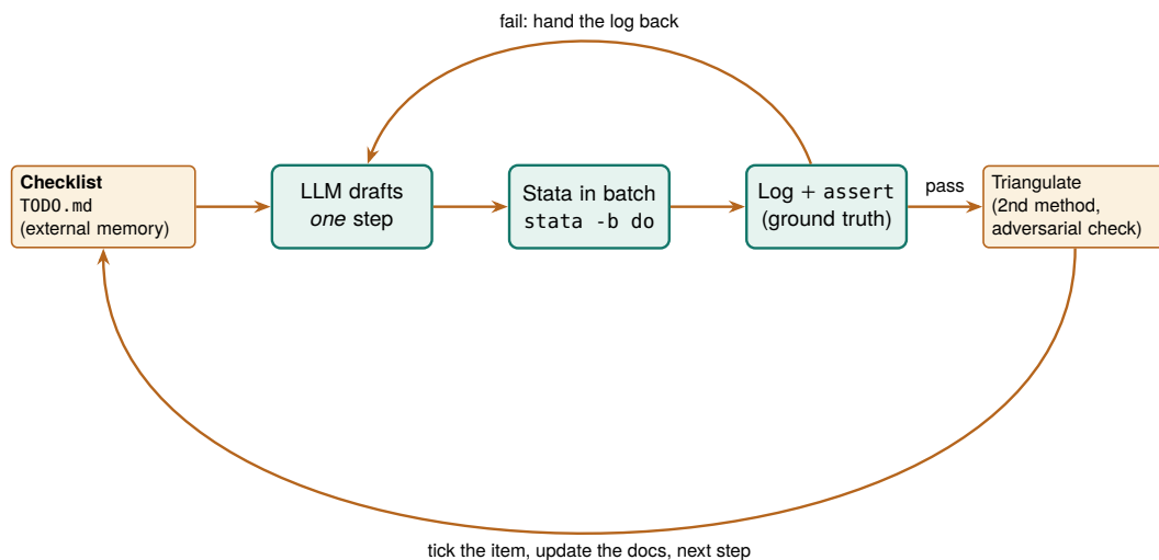
Figure 13.1: The backbone loop. An external checklist holds the plan; the model drafts one step at a time; Stata runs it in batch and the log, with assert tripwires, is the only thing trusted to say the step worked; a failing step hands the log back to the model to fix; a passing step is triangulated against a second method, then the checklist and the running documentation are updated before the next step. The model never holds the results; the files do, which is what lets you step in at any point.
