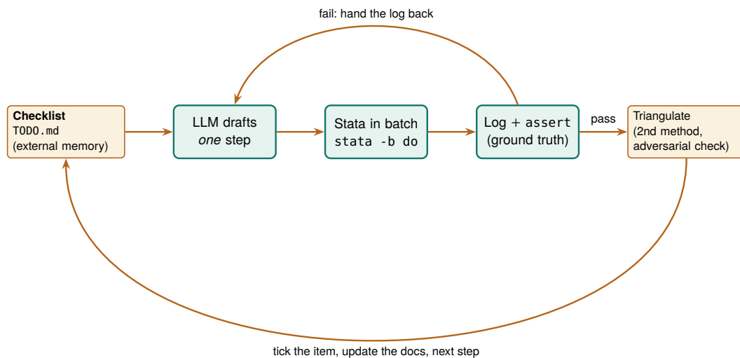
Figure 13.1: The backbone loop. An external checklist holds the plan; the LLM drafts one step at a time; Stata runs it in batch and the log, with assert tripwires, is the only thing trusted to say the step worked; a failing step hands the log back to the LLM to fix; a passing step is triangulated against a second method, then the checklist and the running documentation are updated before the next step. The LLM never holds the results; the files do, so you can step in at any point.
