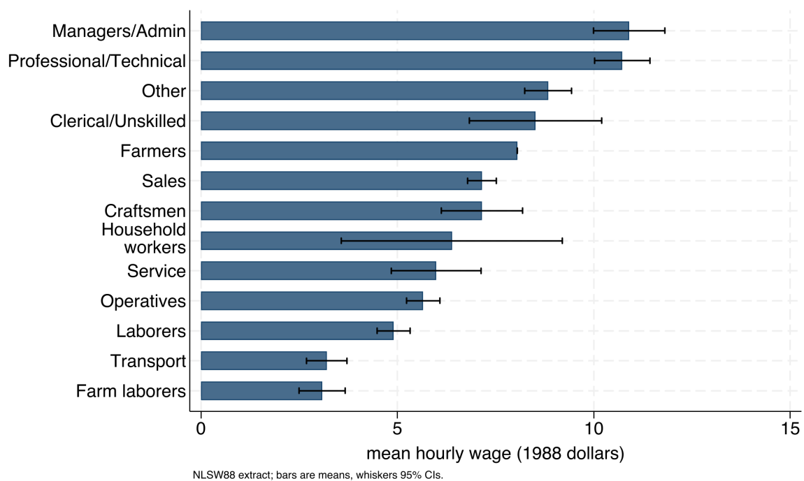
Figure 9.4: Mean hourly wage across thirteen occupations in the nlsw88 extract, drawn by one statplot call with ci sort wrap(14) : categories ranked by the statistic, labels wrapped, and a 95 percent interval wherever the data can support one. Managers/Admin tops the ranking at $10.90 and farm laborers close it at $3.08. The intervals carry the caution the ranking needs: household workers ( N = 2 ) spans $3.58 to $9.20, and the single-observation farmers category collapses to a bare tick at the mean, so the eye sees at once which positions rest on real support. Built by ch09_graphs.do .
