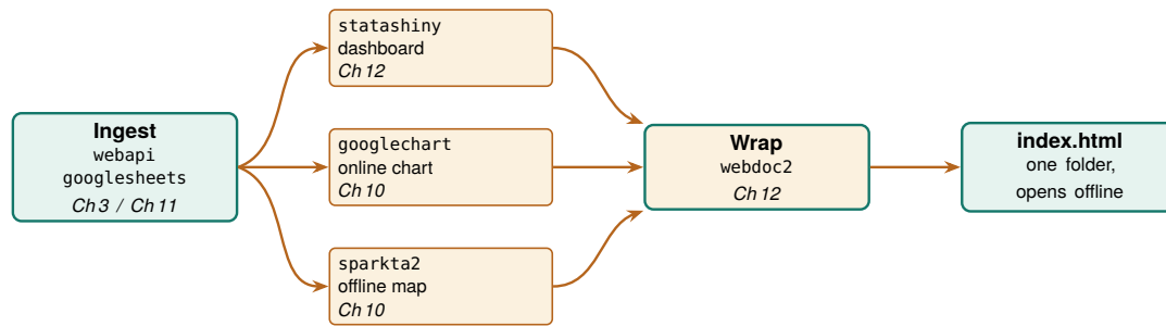
Figure 12.2: The suite as one pipeline. webapi or googlesheets ingests the data; googlechart renders an online interactive chart, sparkta2 an offline map, and statashiny an interactive dashboard; webdoc2 wraps all three into one index.html that opens offline from a single folder. Each box names the chapter that teaches it. The companion ch12_portal.do walks these same arrows in code.
