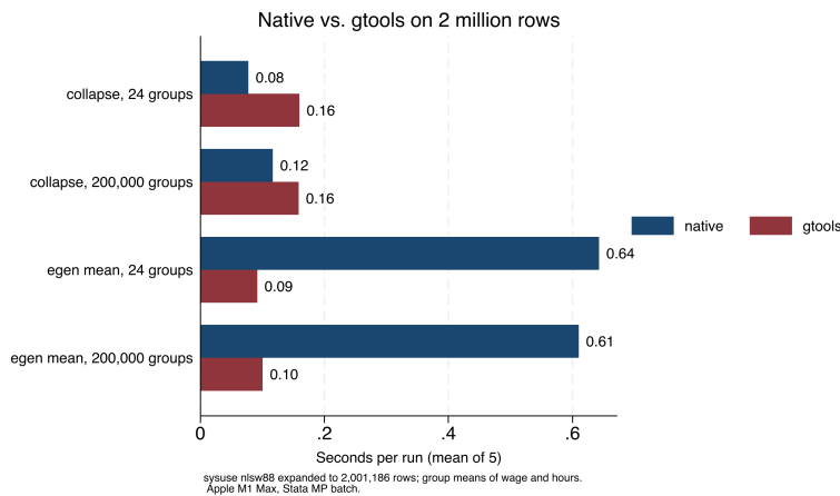
Figure 2.4: Seconds per run for four operations on a simulated two-million-row file, native Stata versus gtools, mean of five runs on an Apple-silicon Mac in Stata MP. gtools wins by roughly seven-fold on egen, where the native command is slow, and loses slightly on collapse, where the native command is already fast. The bars and Table 2.2 carry the same numbers: benchmark before you optimize.
