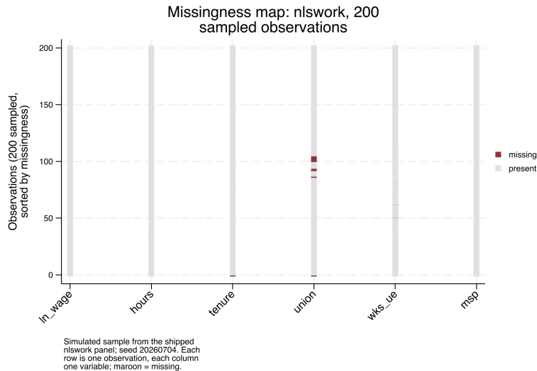
Figure 6.3: Missingness map for 200 observations sampled (seed 20260704) from the shipped nlswork panel. Each row is one observation, each column one variable; maroon marks a missing cell and rows are sorted by how much is missing. The gaps cluster in union and wks_ue , while ln_wage , hours , tenure , and msp are effectively complete, which matches the misstable patterns table and tells you casewise deletion here would drop rows on those two variables, not at random. Built by ch06_longitudinal.do ; the command is printed above it.
