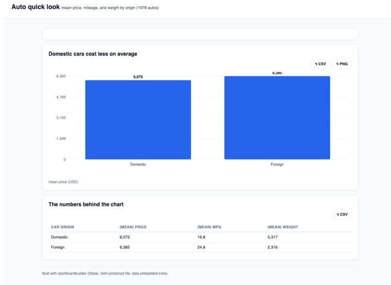
Figure 12.1: The two-minute build: one init, two panel calls, one build, and the result is a single HTML file with the data inlined. The CSV and PNG buttons on each panel are defaults, so every chart ships its own numbers. Built by the companion ch12_dashboardbuilder.do .
