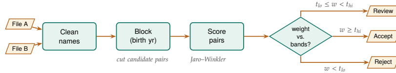
Figure 6.1: The probabilistic-linkage pipeline the section walks: two source files are name-cleaned, blocked on a reliable key to cut the candidate pairs, scored with a string comparator, then split by match weight into three bands. See that the middle band routes to human review rather than a silent accept or reject, and that only the scoring box changes when you swap comparators.
