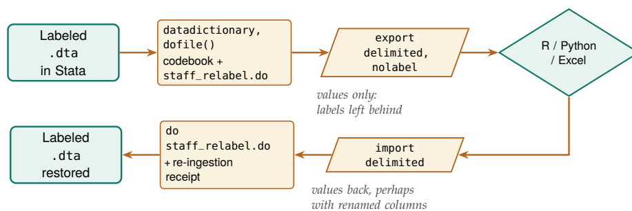
Figure 5.4: Data leaves Stata as bare values and returns re-dressed. datadictionary writes the codebook and a capture-guarded relabel do-file; export delimited, nolabel sends numeric codes a collaborator edits in R, Python, or Excel; on return, do staff_relabel.do restores every label, format, note, and characteristic and prints a receipt naming any column that was renamed, dropped, or added. Export with nolabel so value labels have codes to reattach to.
