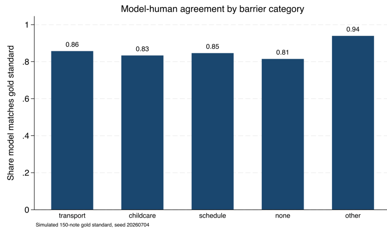
Figure 13.2: Share of notes on which the simulated model matches the hand-coded gold standard, one bar per barrier category (150 simulated notes, seed 20260704). Overall agreement is high, but the “none” category is weakest at 0.81, which is exactly where you spot-check the model and where a consensus tool routes cases to a human. A single kappa would have hidden this.
