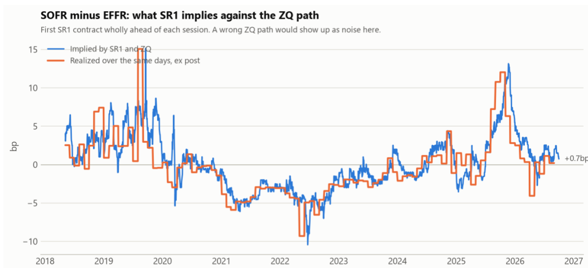
Figure 2. The SOFR – EFRF basis implied jointly by SR1 and the ZQ path.
