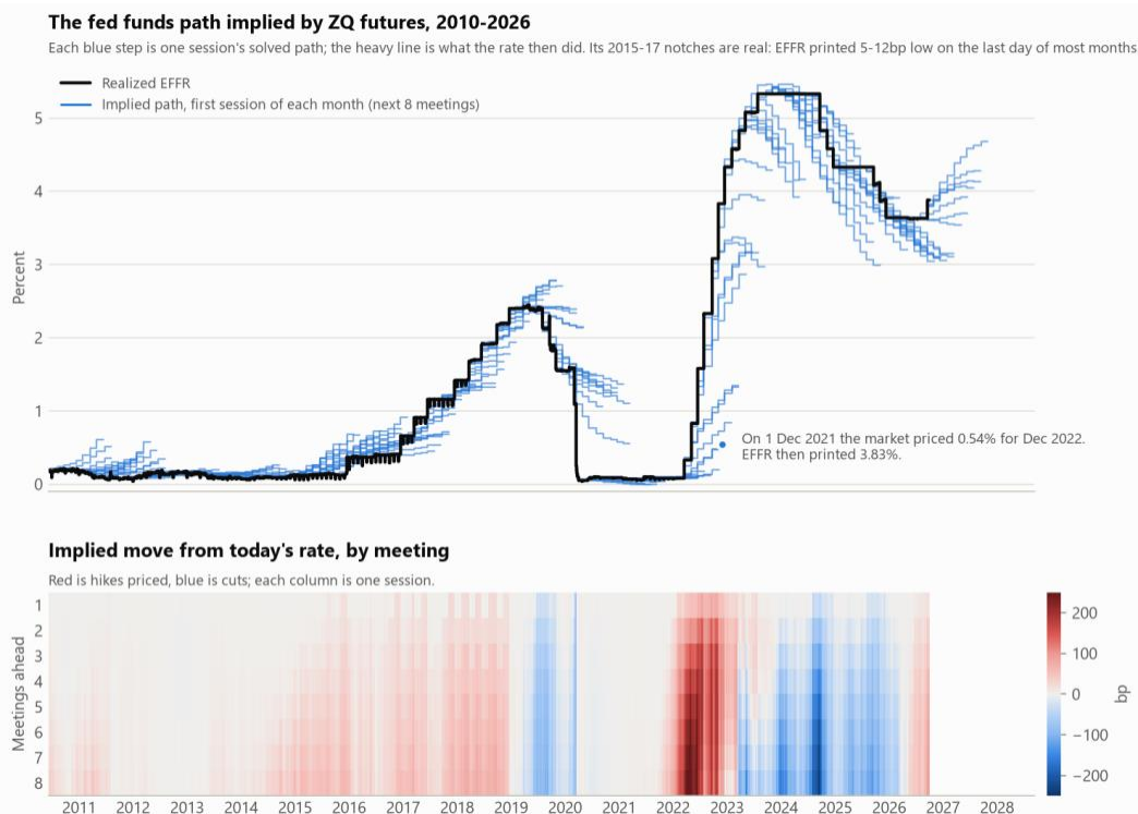
Figure 1. The fed funds path implied by ZQ futures, and the move priced at each meeting.
