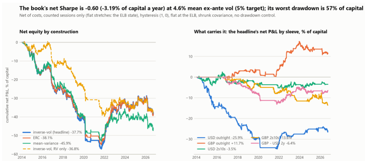
Figure 8. Net equity of the book by construction, and the headline book's net P&L by sleeve.
