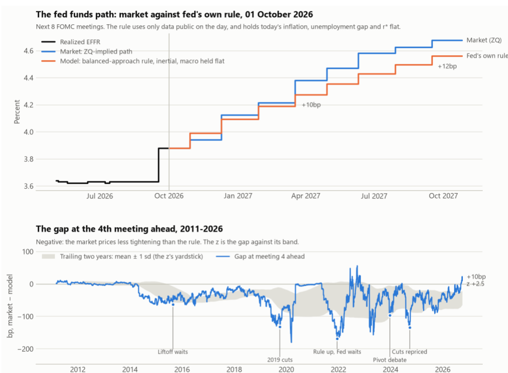
Figure 5. USD: the market path against the balanced-approach rule, and the gap at the fourth meeting ahead.
