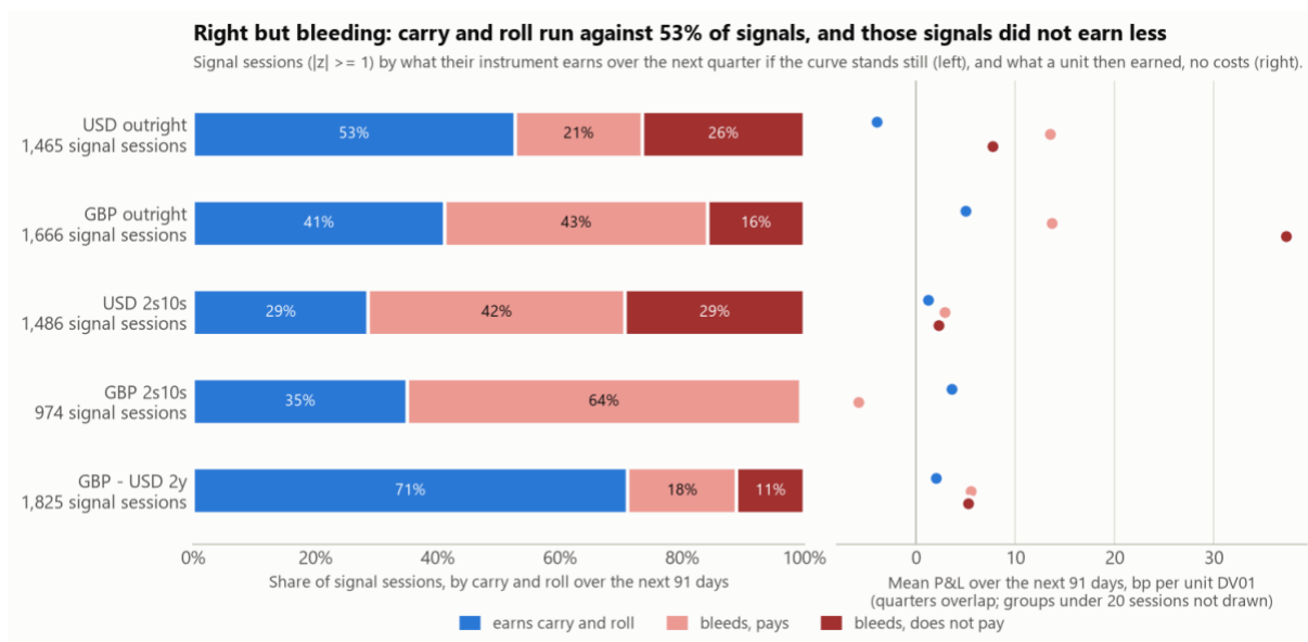
Figure 11. Carry and roll against the side held, by sleeve, and what those signals earned.
