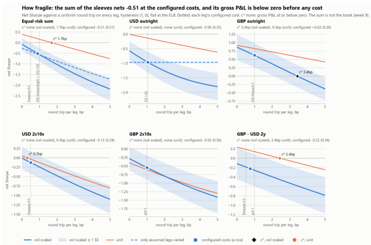
Figure 13. Net Sharpe ratio against a uniform round-trip cost, by sleeve (the sum of the sleeves, not the book).
