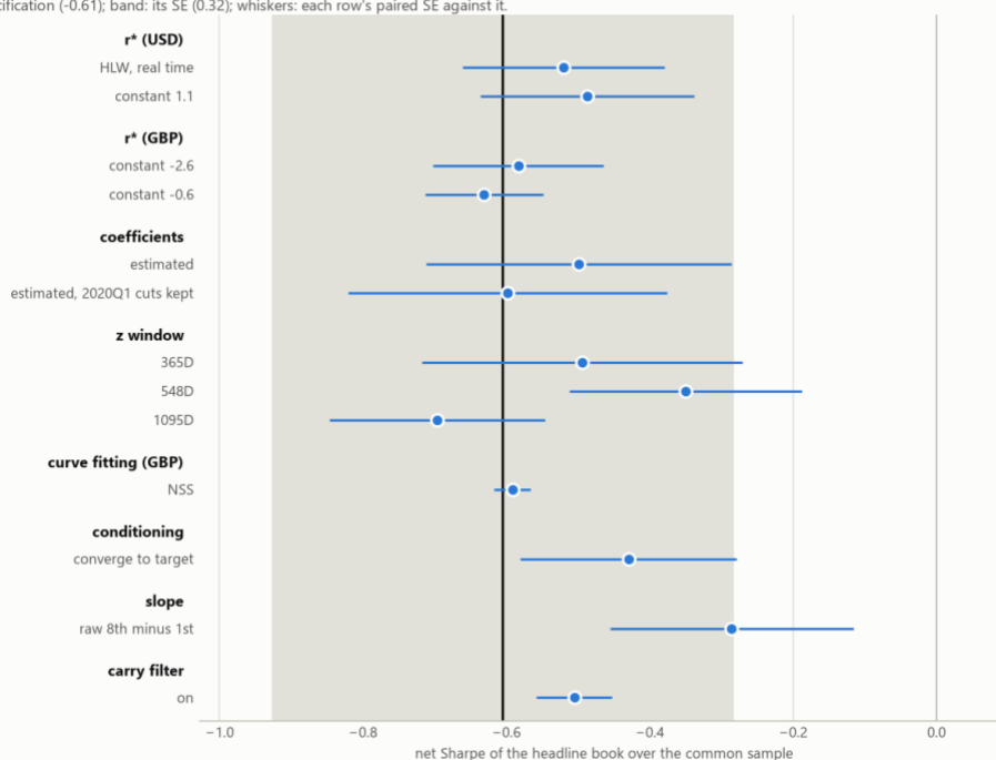
Figure 12. The headline book's net Sharpe ratio with one choice at a time moved off the chosen specification.
