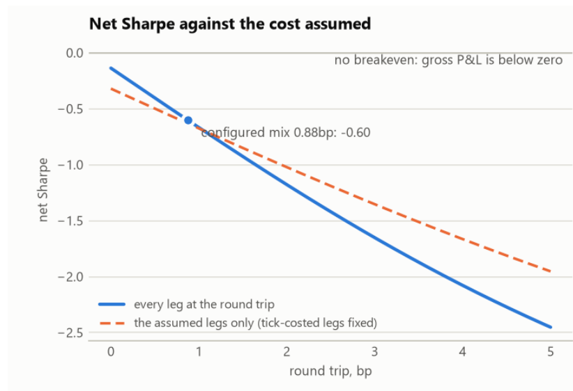
Figure 10. The book's net Sharpe ratio against the round-trip cost assumed.
