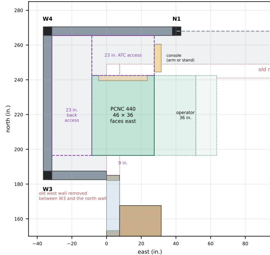
PCNC 440 — Option 3: 23 in. off the walls, operator in the room
