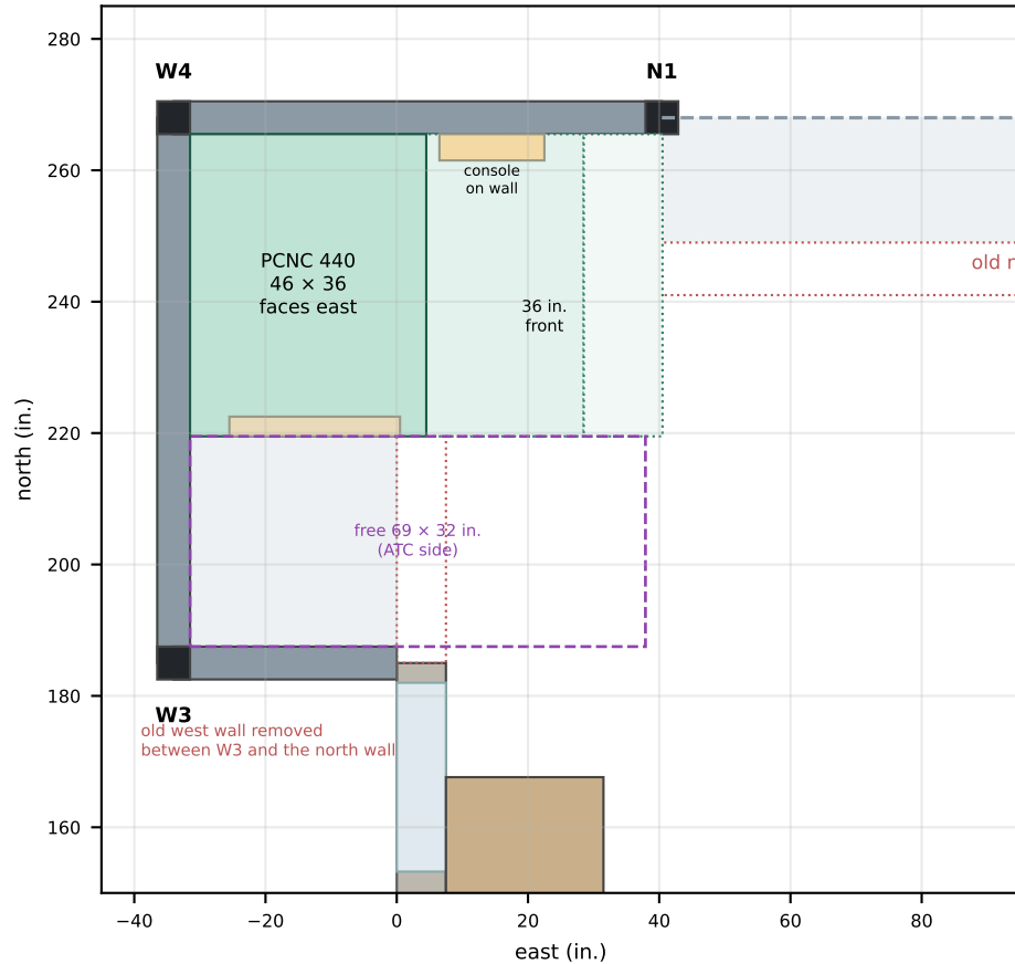
PCNC 440 — Option 1: against the walls, faces east
