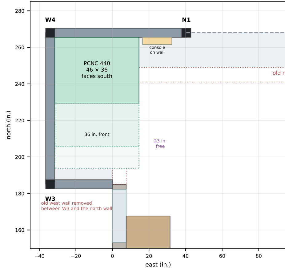
PCNC 440 — Option 2: against the walls, faces south
