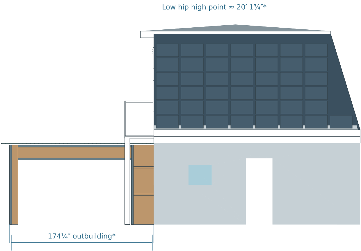
03 South elevation · looking north
