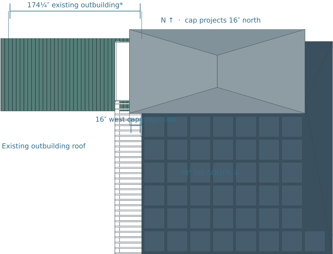
02 Roof plan · north up
