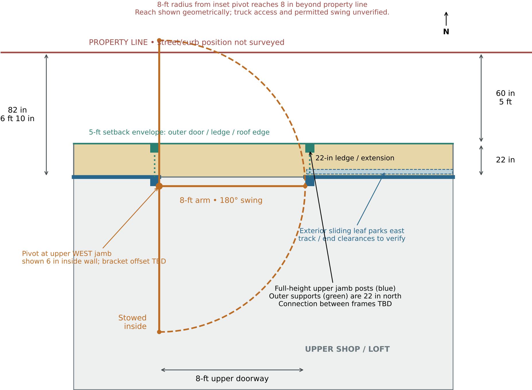
UPPER-FLOOR PLAN — north up, west left
