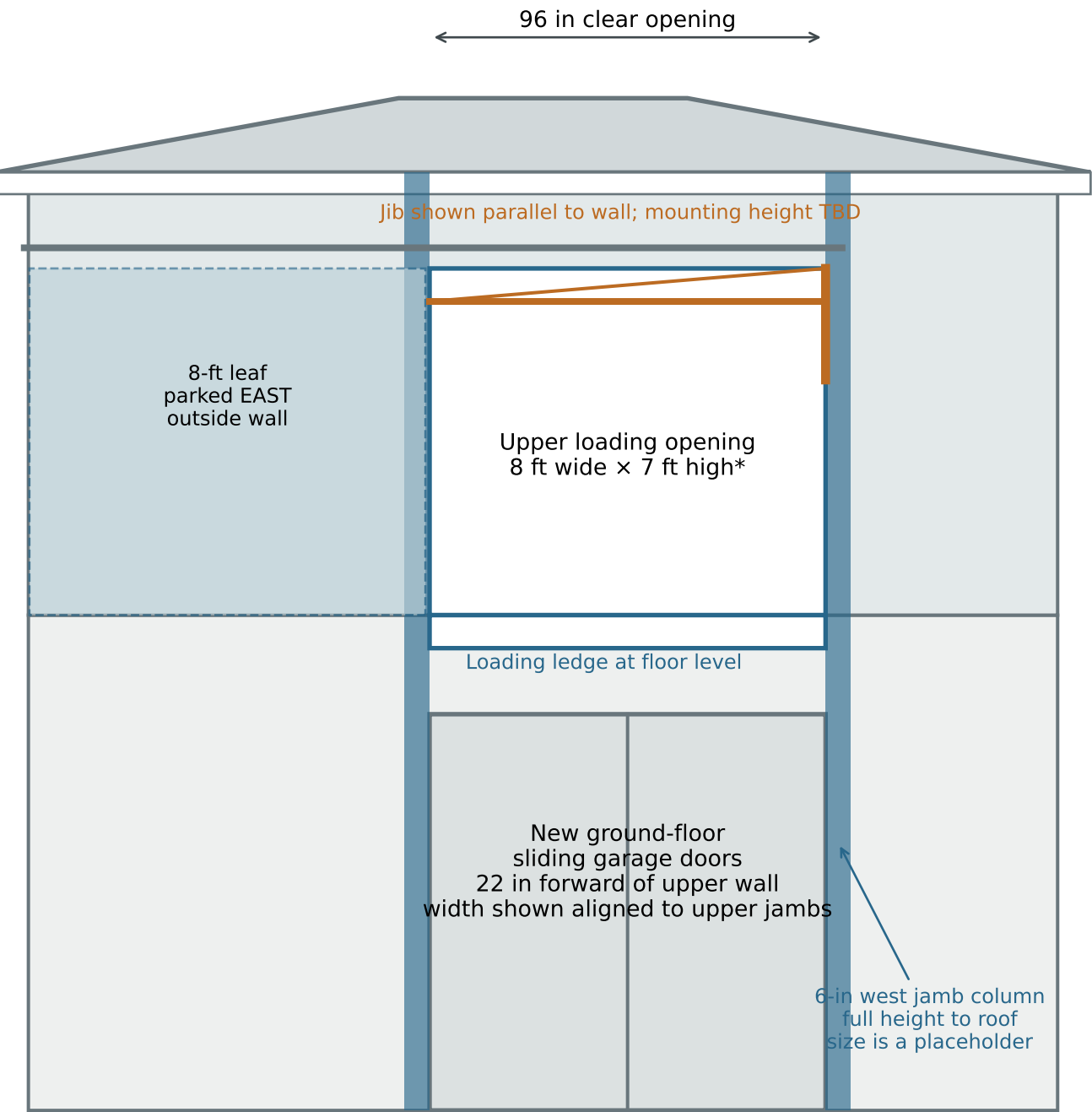
NORTH ELEVATION — conceptual placement
