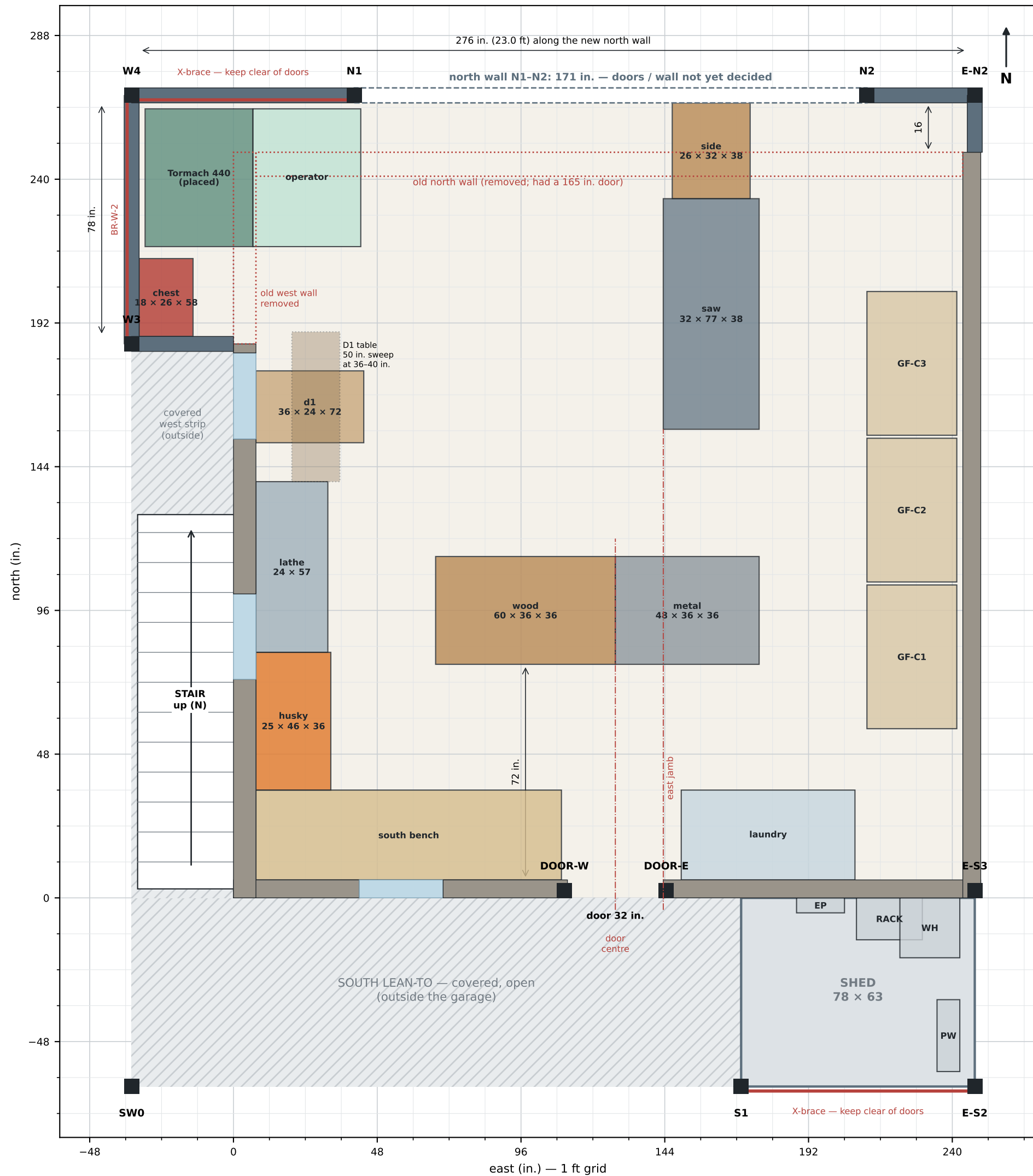
Ground floor — equipment layout (plan from above) labels: E-W x N-S x height, in. · dotted = D1 table sweep
