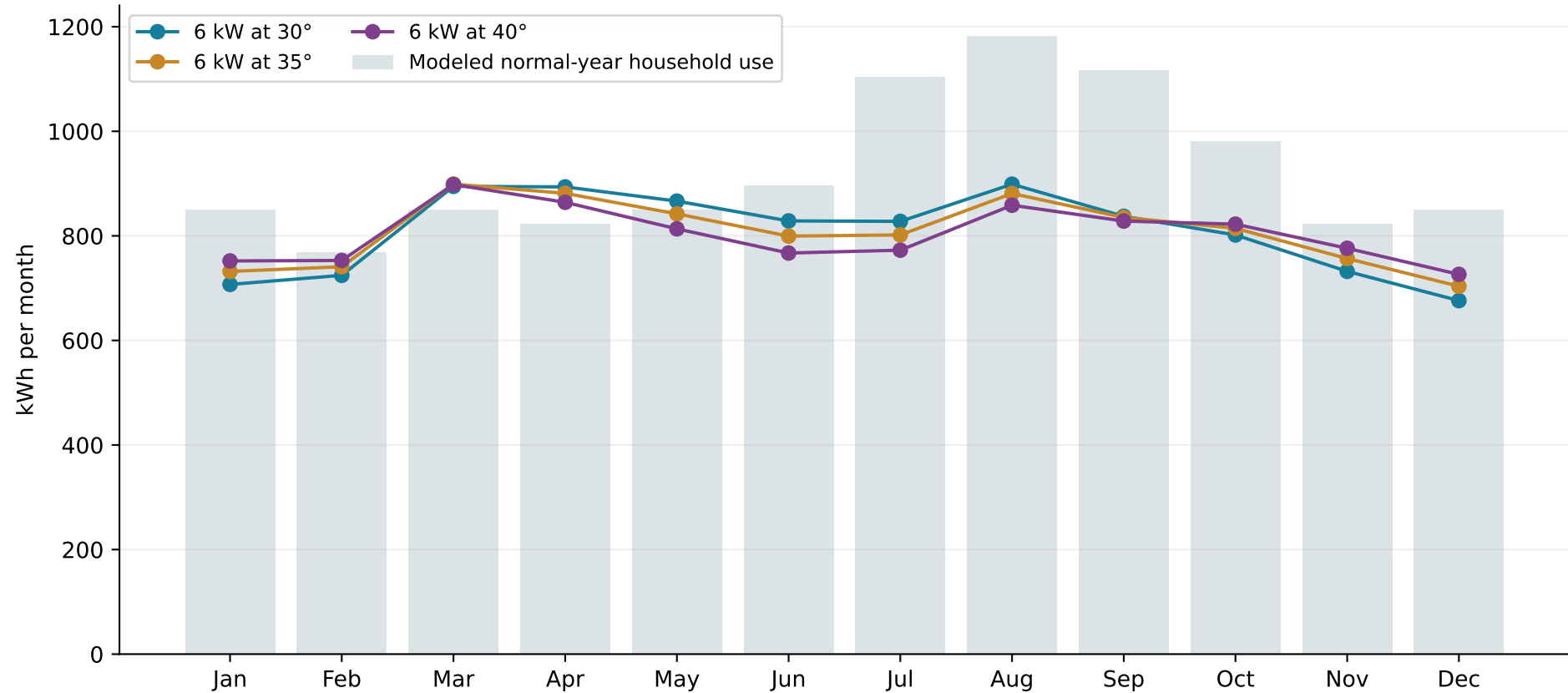
Same 6 kW array: tilt shifts energy toward winter
