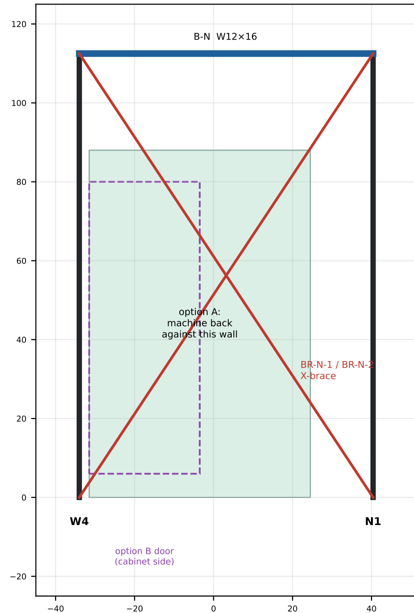
North wall W4-N1, looking north from inside
