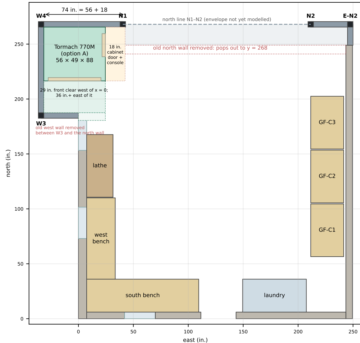
Ground floor with the NW pop-out (W3-W4-N1) and north wall at y = 268
