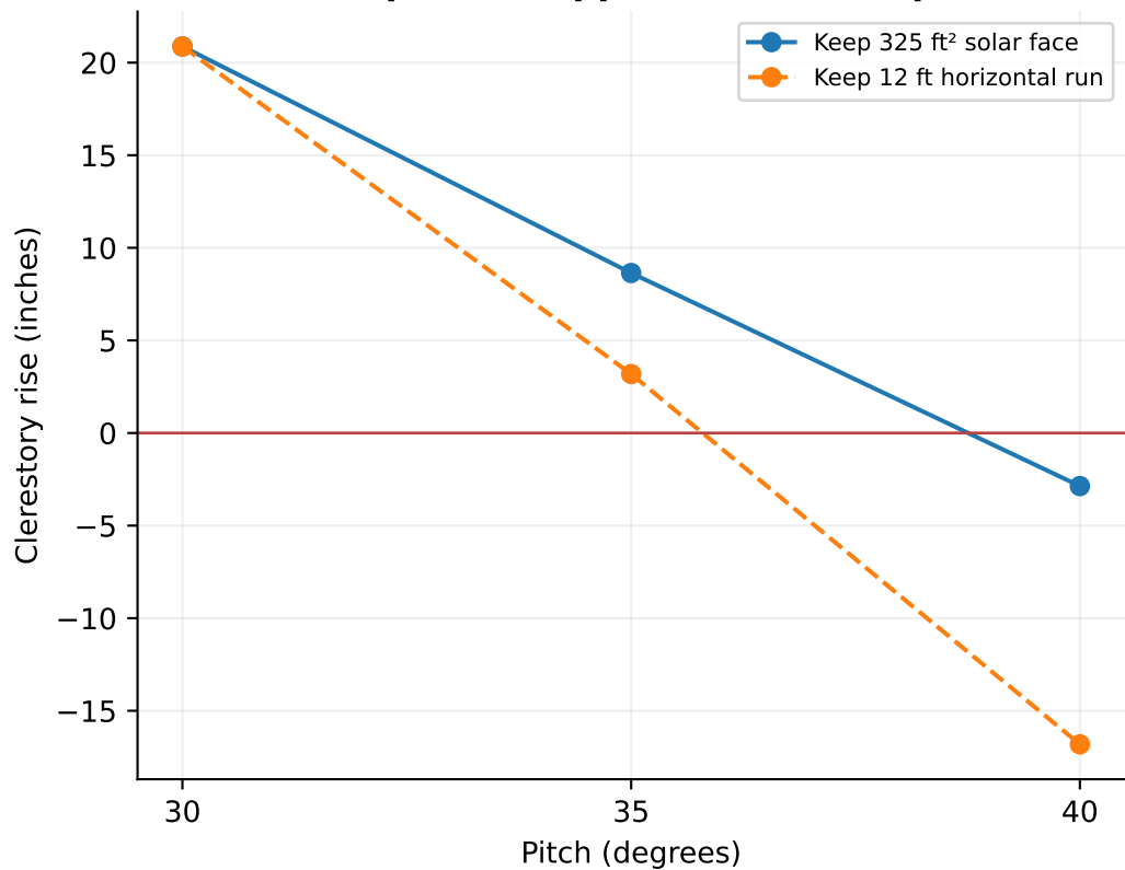
Window space disappears as the slope rises
