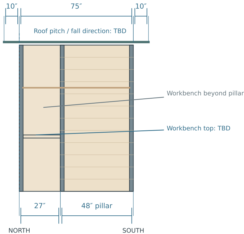
03 WEST ELEVATION · looking east
