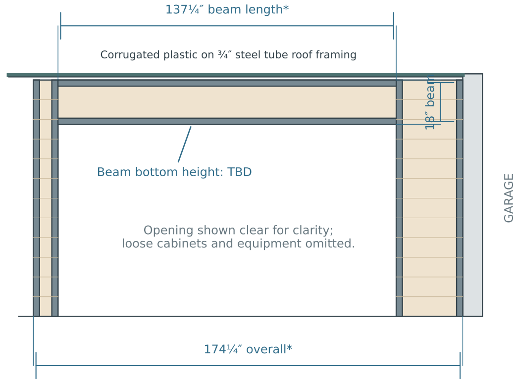
02 SOUTH / FRONT ELEVATION · looking north
