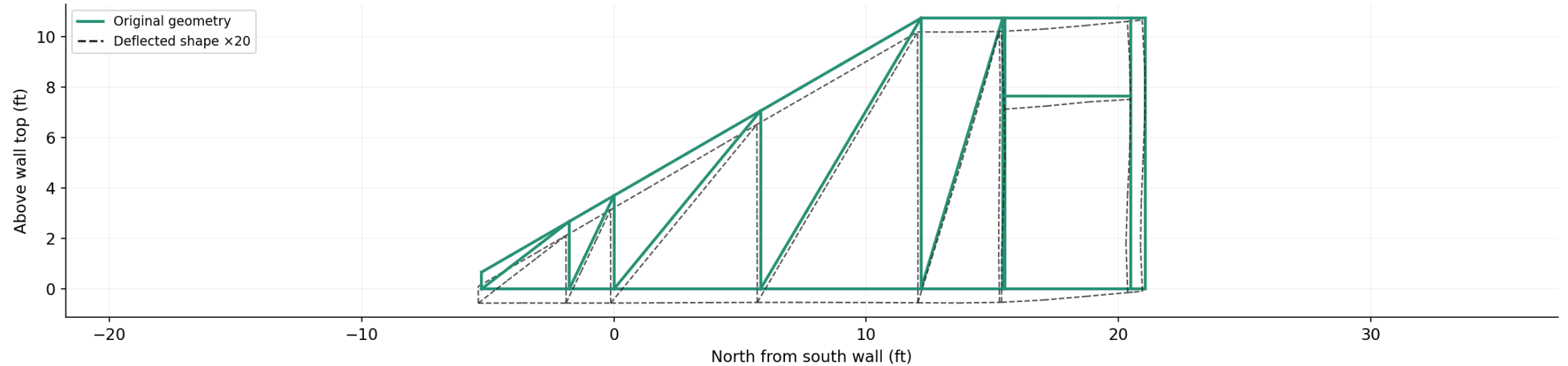
T-W — west longitudinal TRUSS
