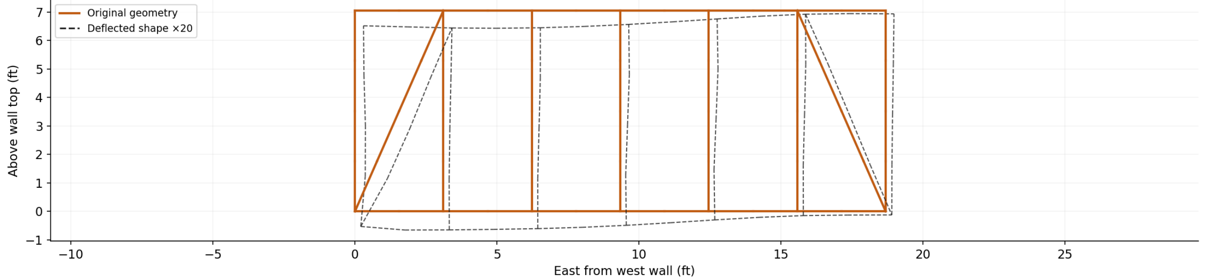
T-E — east longitudinal TRUSS
