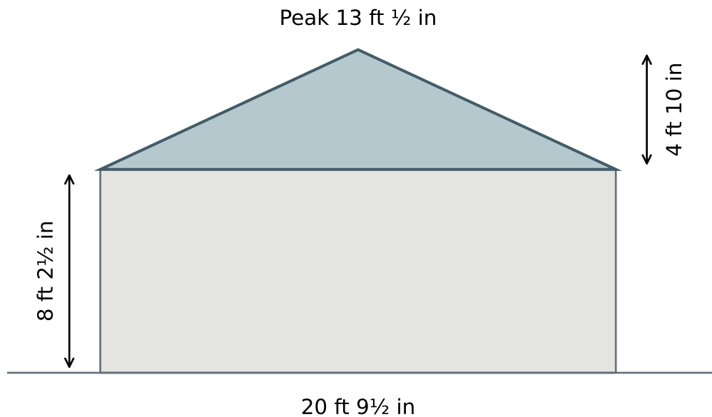
South elevation
