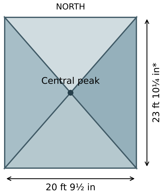
Roof plan · four triangular faces
