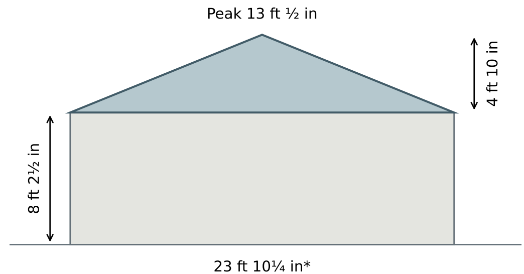
West elevation
