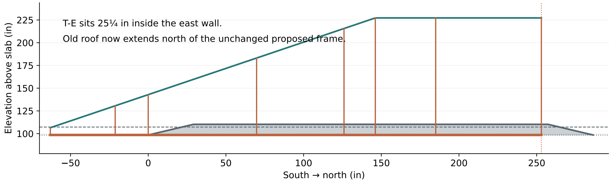
T-E section · looking west · X = 224.25 in
