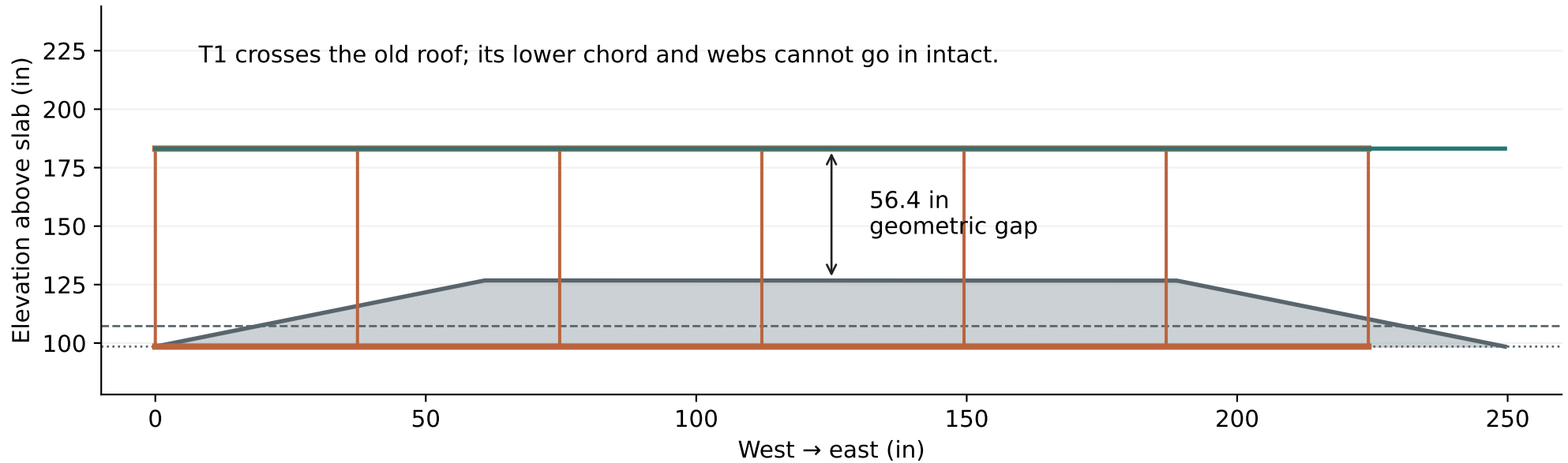
T1 section · looking north · Y = 69.75 in
