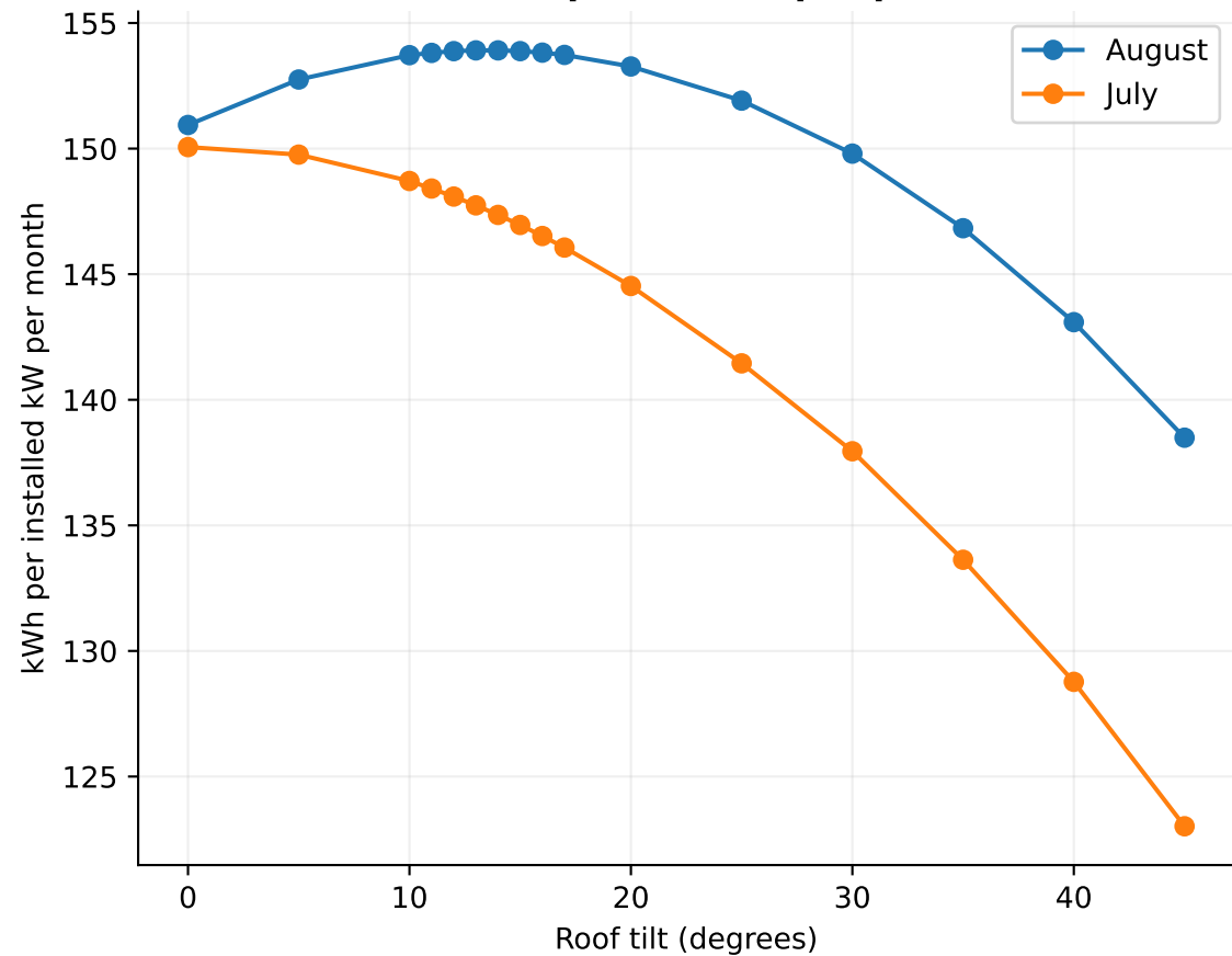
Summer production per panel
