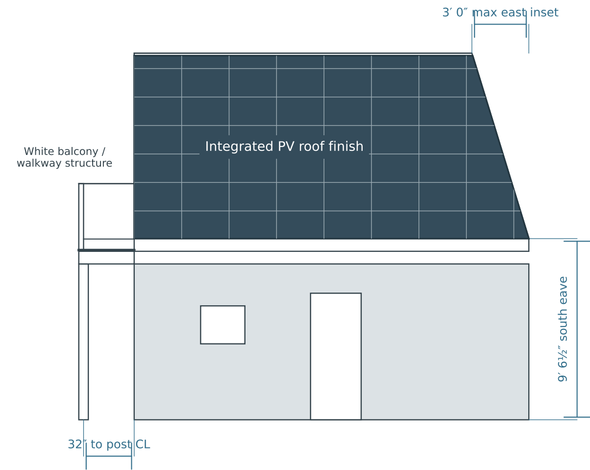
02 SOUTH ELEVATION · looking north
