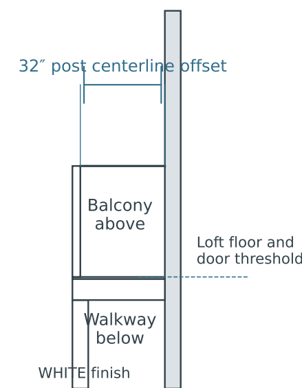
03 WEST WALKWAY / BALCONY SECTION · diagram
