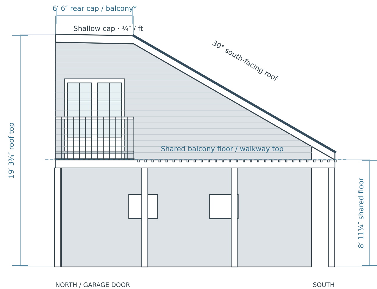
01 WEST ELEVATION · looking east
