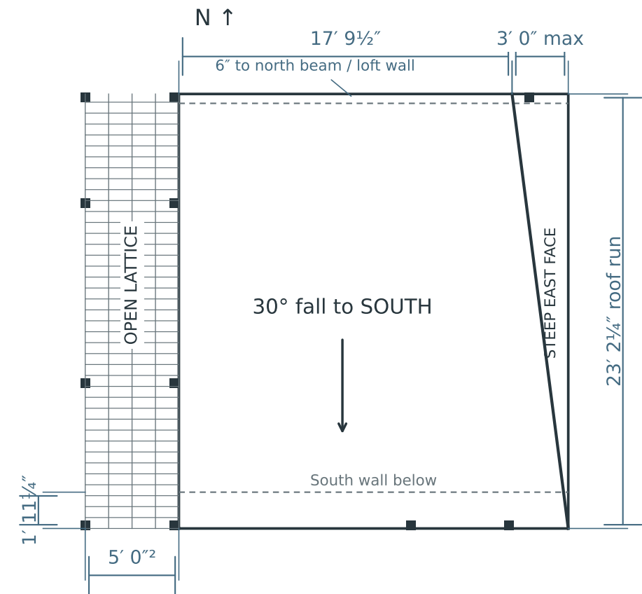
02 Roof plan · north up
