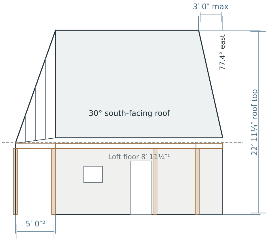
03 South elevation · looking north
