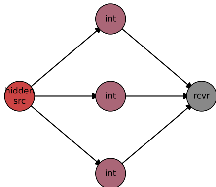
common_source_laundersing
