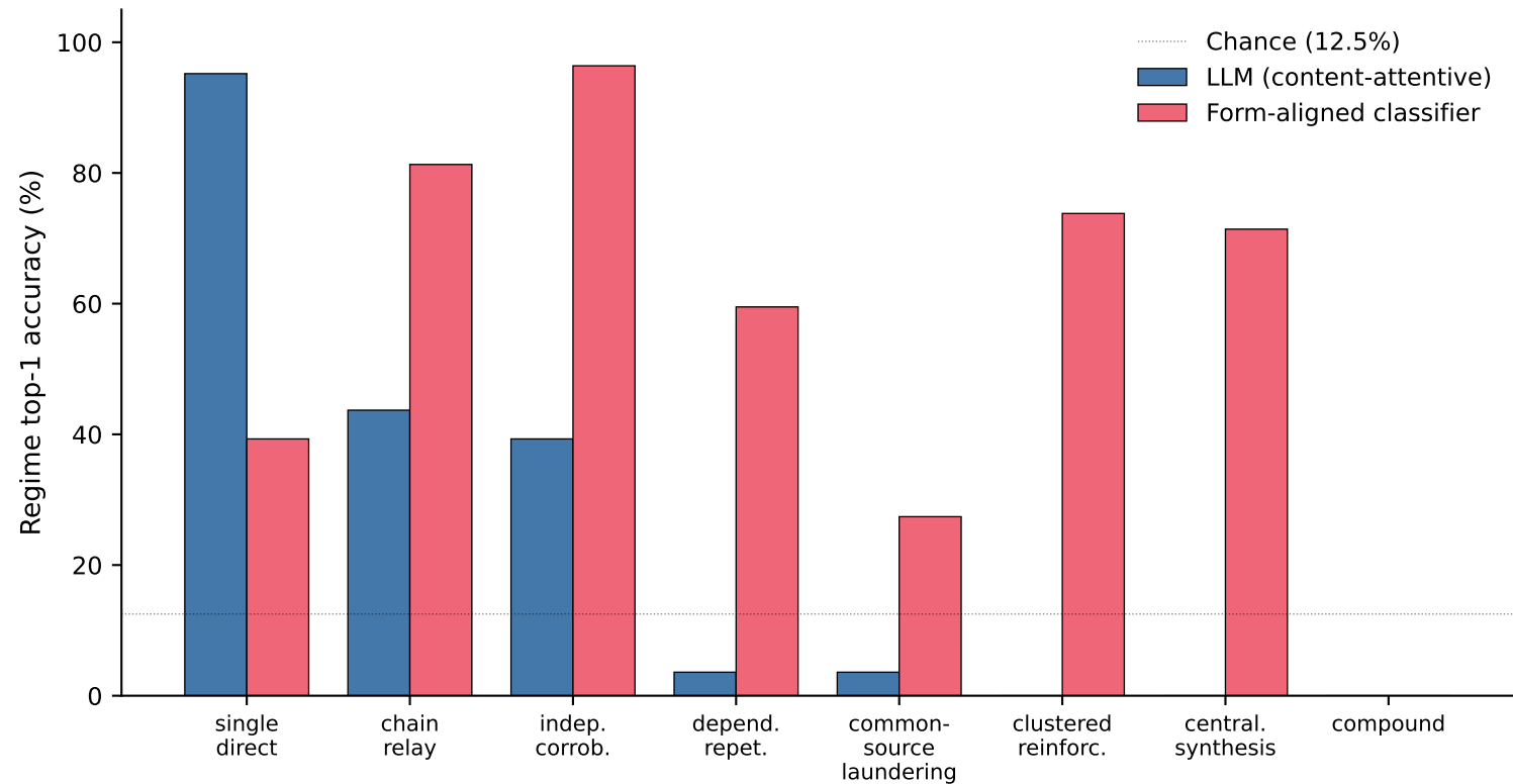
Recoverability by graph motif (F1 primary run, n = 840 test trials)
